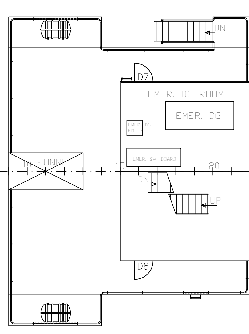
3rd DECK PLAN
