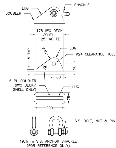
WEB SLING RESTRAINT DETAILS FOR REFERENCE, ADJUST TO SUIT (TYP.) SCALE: 1:10
