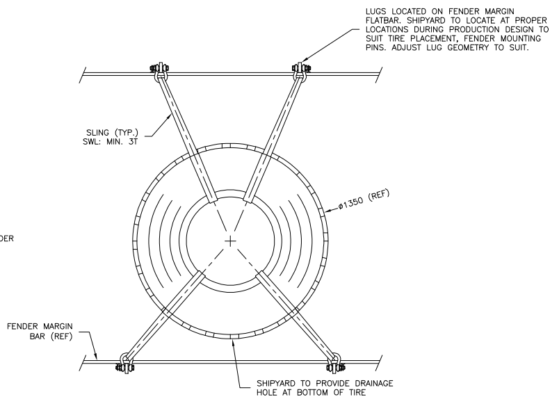
VIEW 'E-1'
