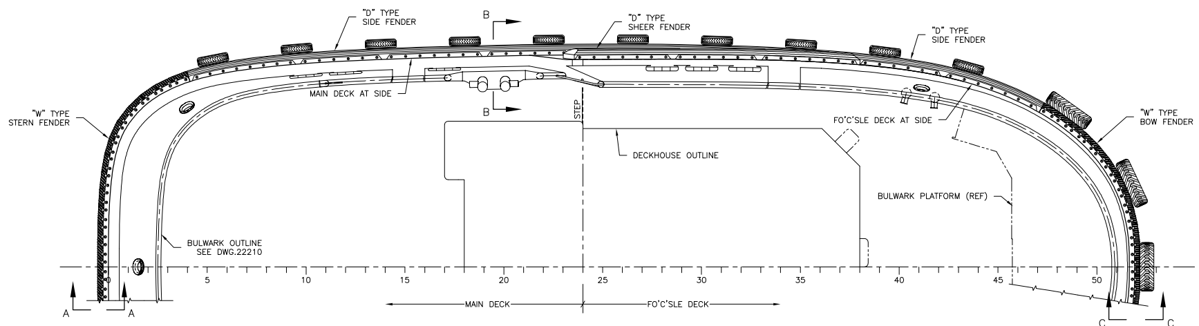
DECK PLAN PORT SIDE SHOWN, STARBOARD SIDE SIMILAR
