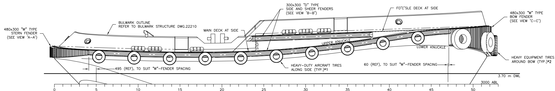
OUTBOARD PROFILE STARBOARD SIDE SHOWN, LOOKING TO PORT PORT SIDE SIMILAR
