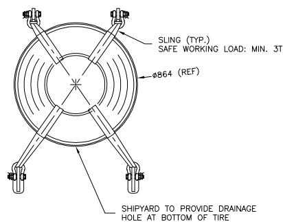
VIEW 'D-1'
