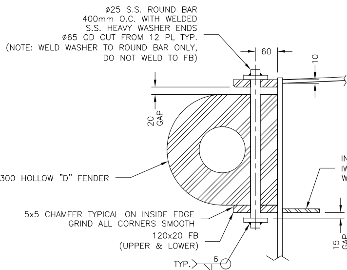
VIEW B-B SHEER 'D'-FENDER
