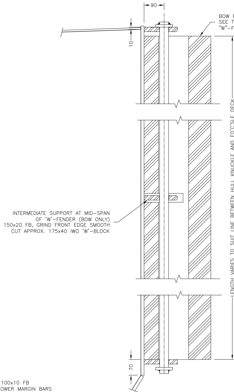
VIEW C-C FORWARD 'W'-FENDER DETAILS SIMILAR TO VIEW 'A-A', UNLESS NOTED OTHERWISE
