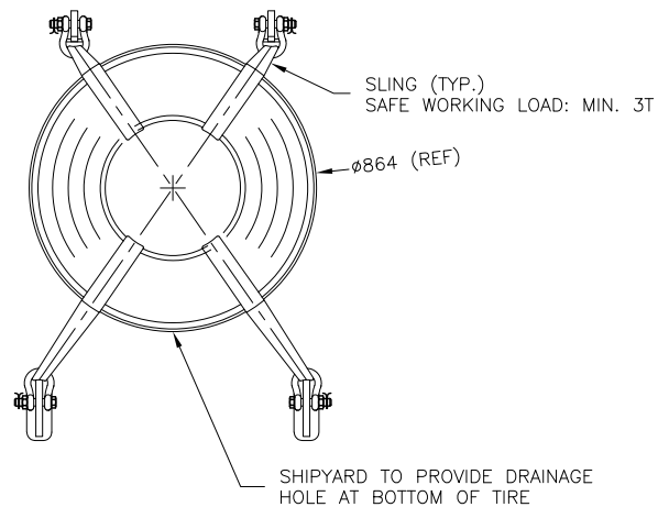
VIEW 'D-1'
