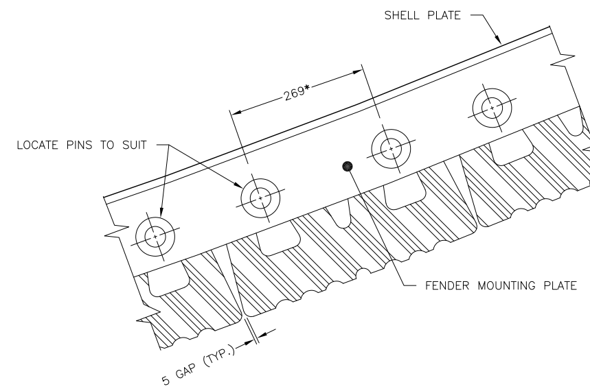
TYPICAL W480x300 MOUNTING PLAN *DIMENSIONS SHOWN FOR REFERENCE ONLY REFER TO FINAL SELECTED EQUIPMENT FOR DETAILS
