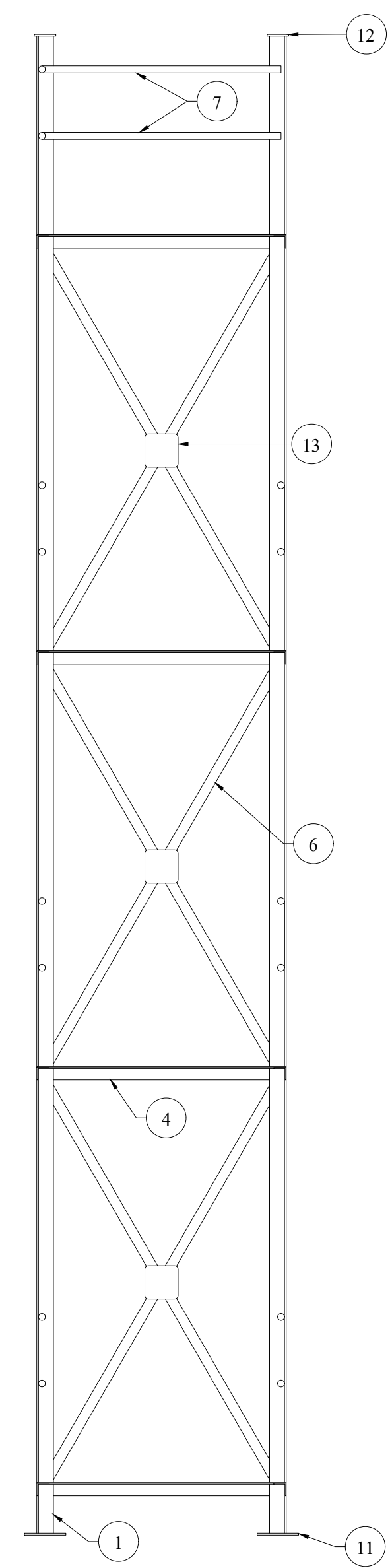
Section F-F
