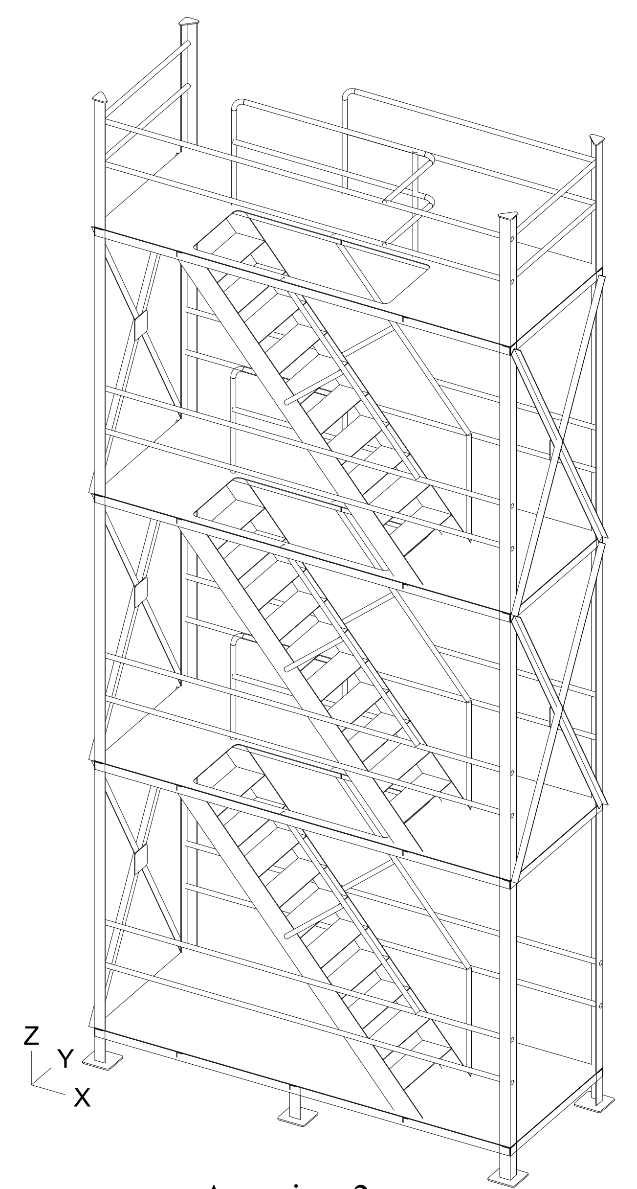
Axo view 2
