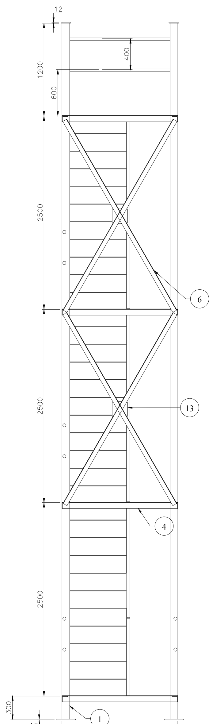
Front view
