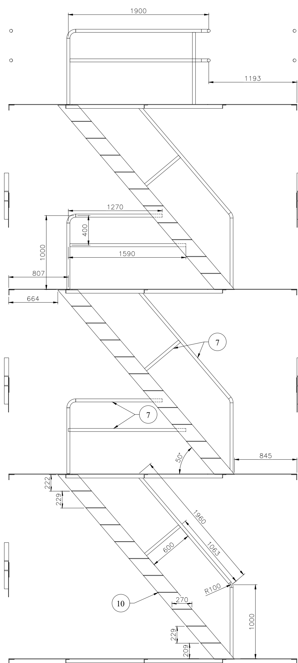
Section B-B
