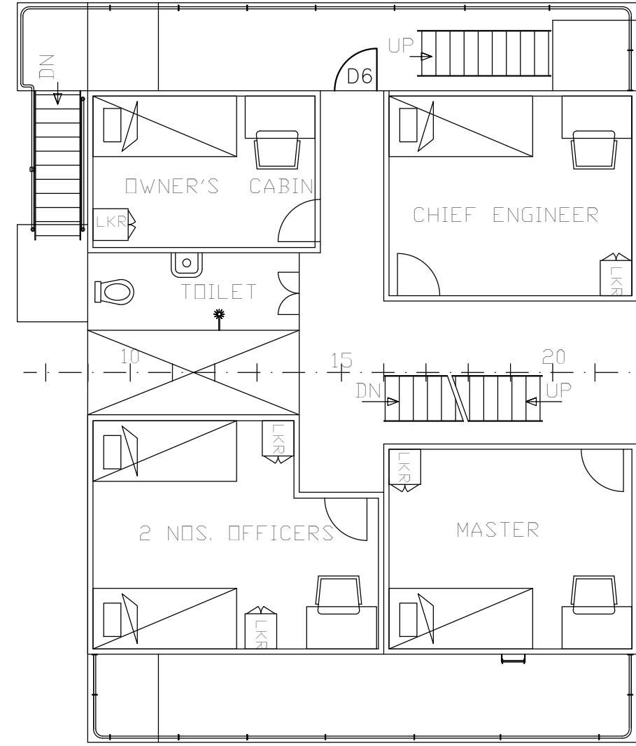
2nd DECK PLAN
