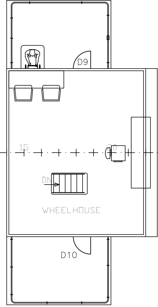
BRIDGE DECK PLAN
