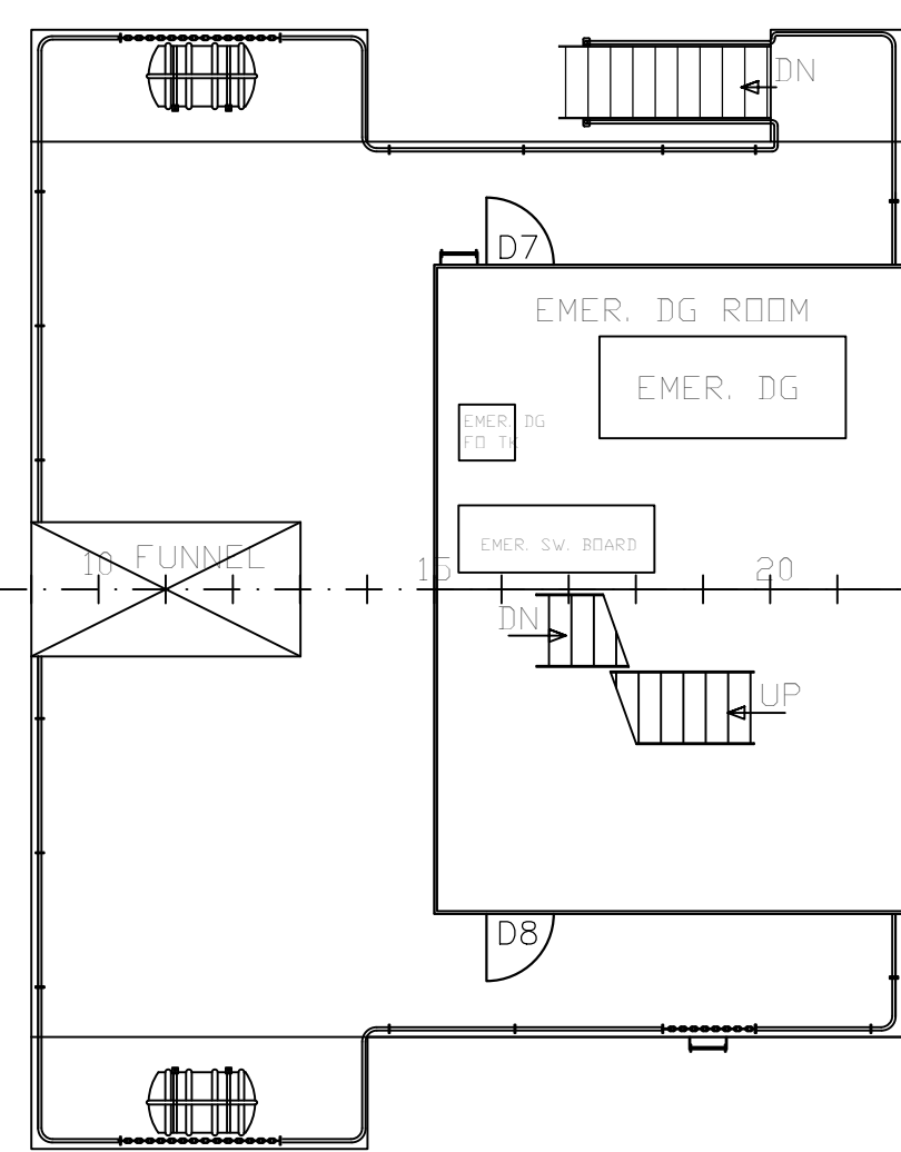
3rd DECK PLAN
