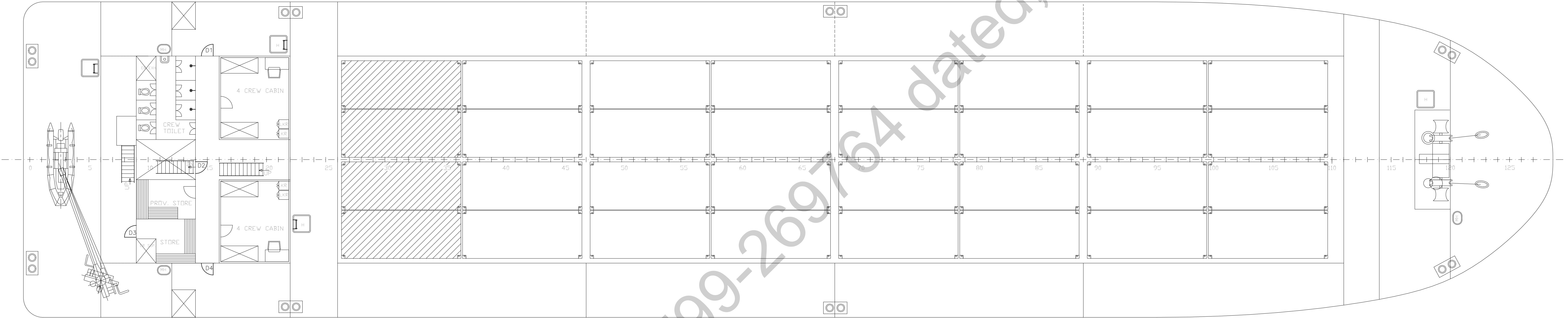
MAIN DECK PLAN
