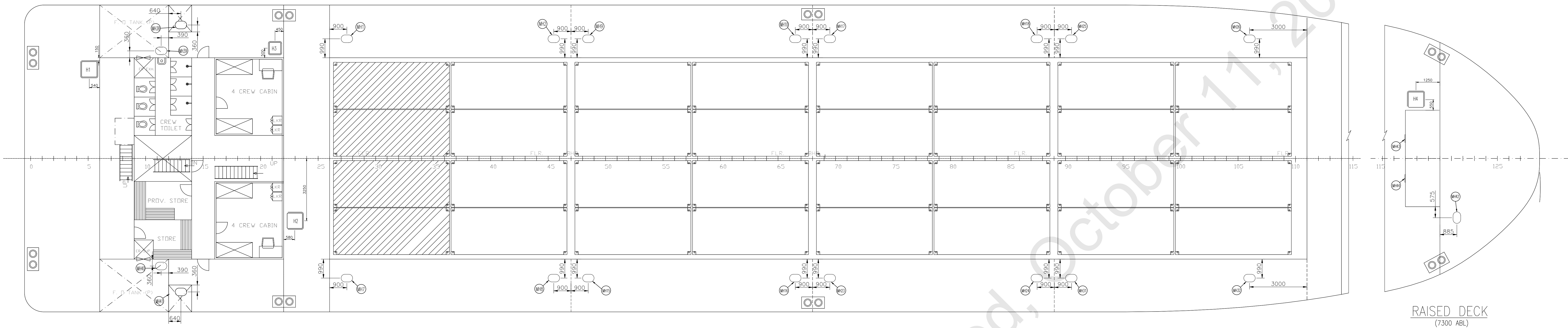
MAIN DECK PLAN
