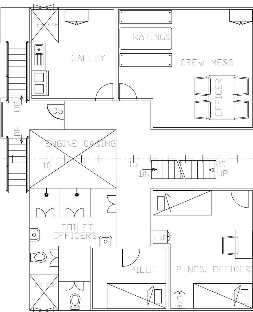
1st DECK PLAN
