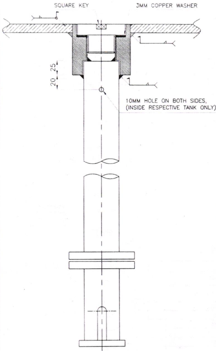
ARRANGEMENT DRAWING (FOR REFERENCE ONLY)
