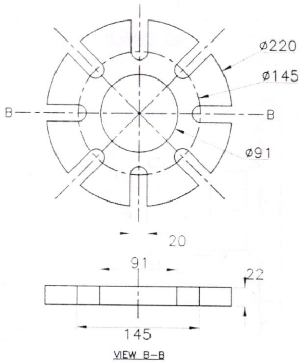
SHORE CONNECTION FLANGE
