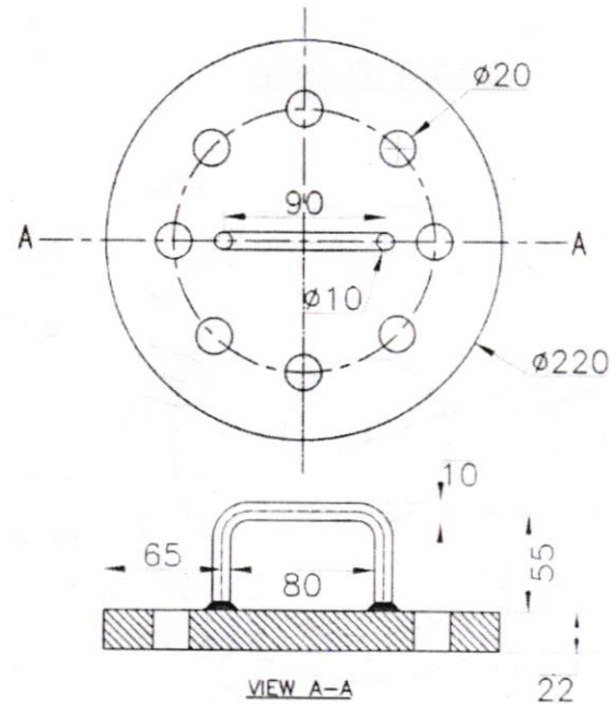
BLIND FLANGE
