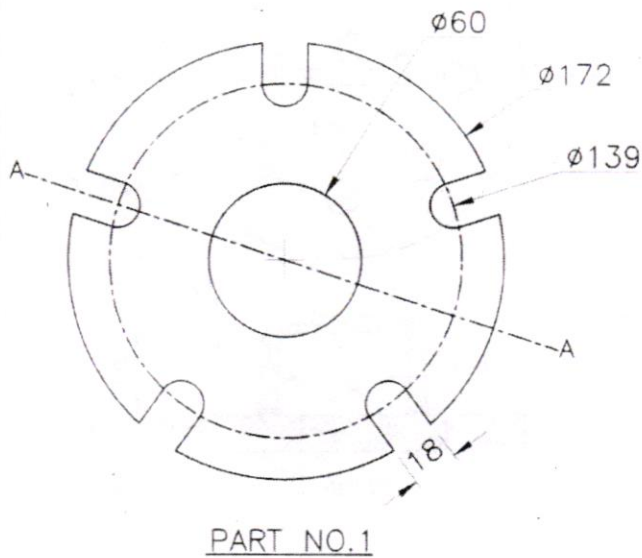
FILLING FLANGE
