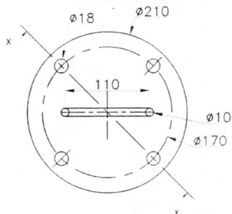
BLIND FLANGE
