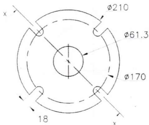
SHORE CONNECTION FLANGE
