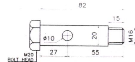
Part 3: M20 BOLT FOR FILLING FLANGE
