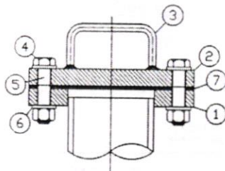
ARRANGEMENT DRAWING (FOR REFERENCE ONLY)
