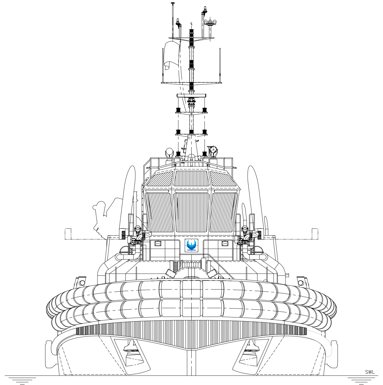
FORWARD VIEW
