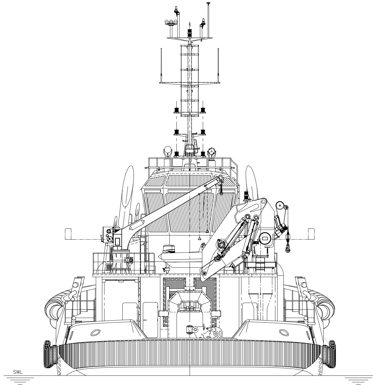
AFT VIEW
