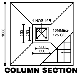
COLUMN SECTION
