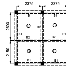
BEAM PLAN
