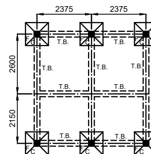
LAY OUT PLAN
