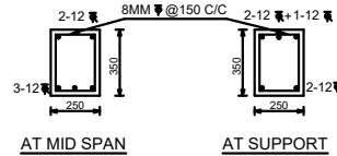
TIE-BEAM (TB)
