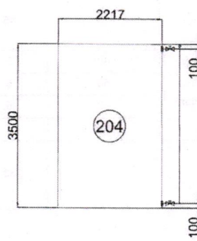
FO SETTLING/DAY TANK
