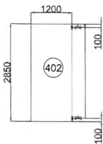
LUBE OIL TANK GEARBOX
