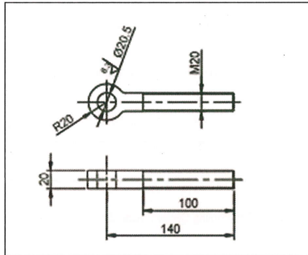
Figure: Eye Bolt (Without collars)
