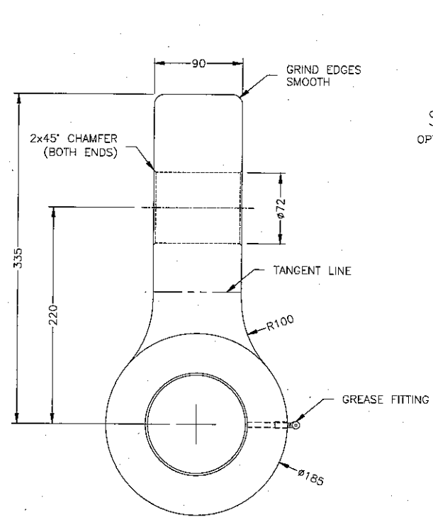
LUG ELEVATION LOOKING PORT (SEE NOTE 1)
