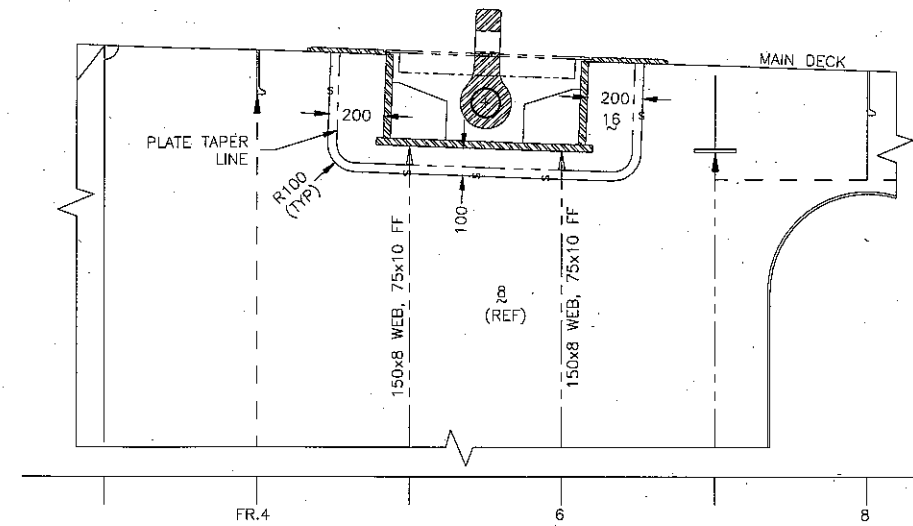
PARTIAL CENTRELINE SECTION
