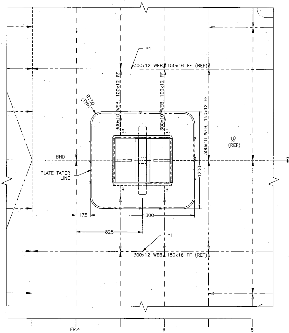
PARTIAL MAIN DECK PLAN SHOWN WITH COVER REMOVED
