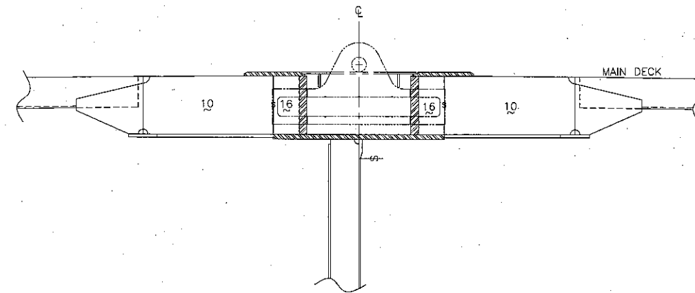
PARTIAL FRAME 6 FRAME 5 SIMILAR UNO
