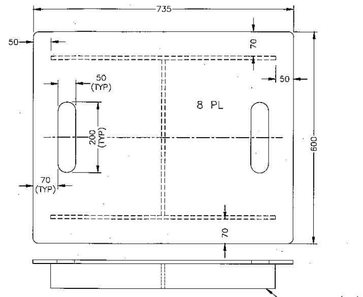
COVER PLATE PROVIDE COVER PLATE INSERT FLUSH TO DECK WHEN GOB EYE IS NOT IN USE. GRIND ALL SHARP EDGES SMOOTH. COAT COVER PLATE TOP WITH NON-SLIP PAINT
