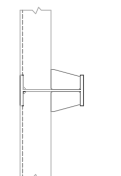
SECTION X-X
