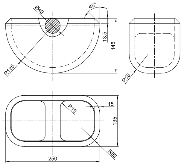
DETAIL OF FLUSH TYPE LASHING POTS (Qty - 244 Nos.)
