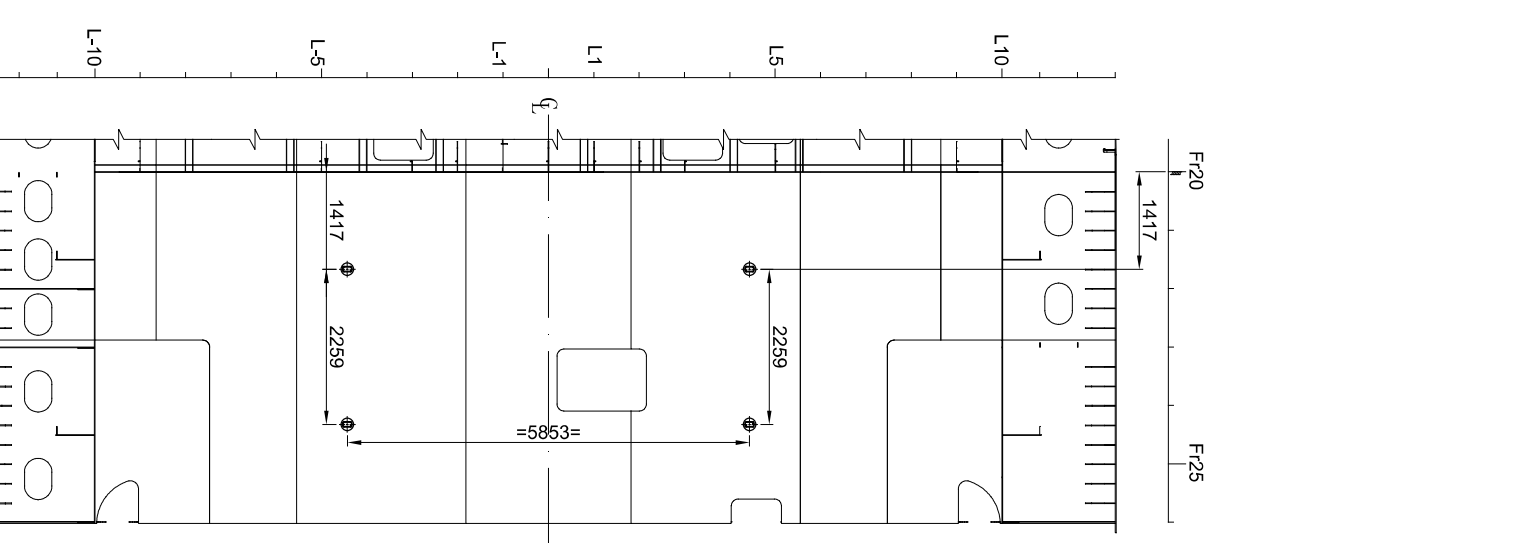
ARRANGEMENT OF LIFTING POCKETS ON TWEEN DECK (Plan View - 6500 ABL)
