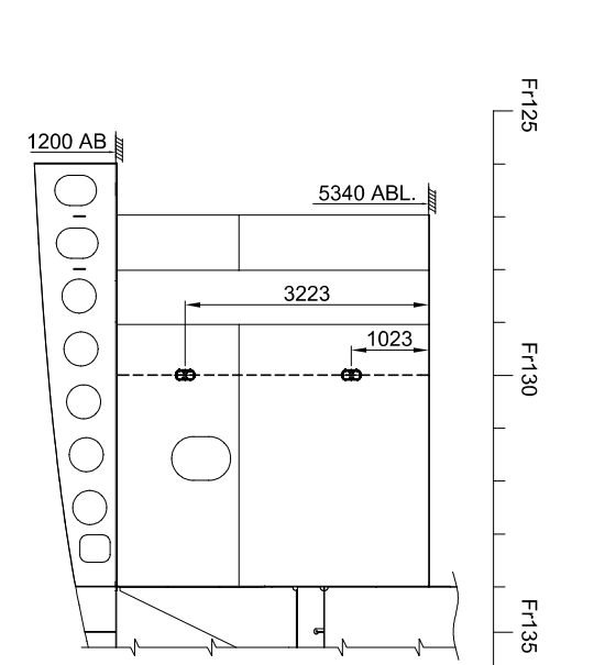
VIEW ON LONG.BHD 3960 off CL (PS Shown, SB Similar)
