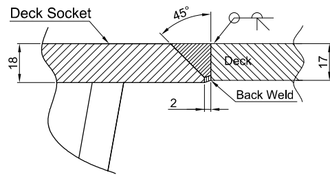
DETAIL - B
