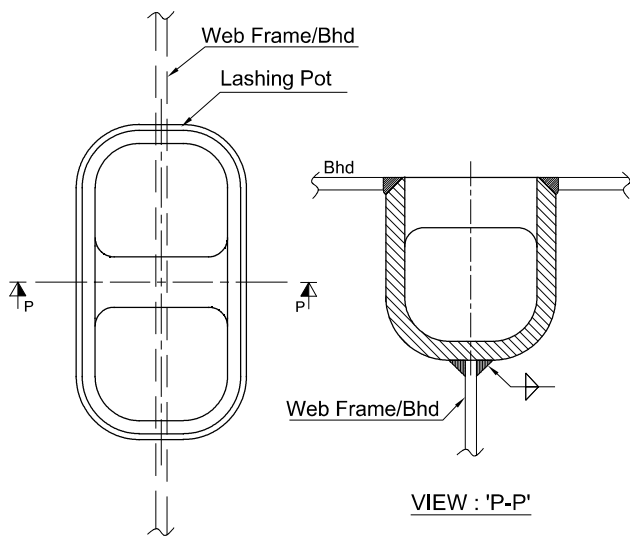
TYP. ARRANGEMENT OF LASHING POT
