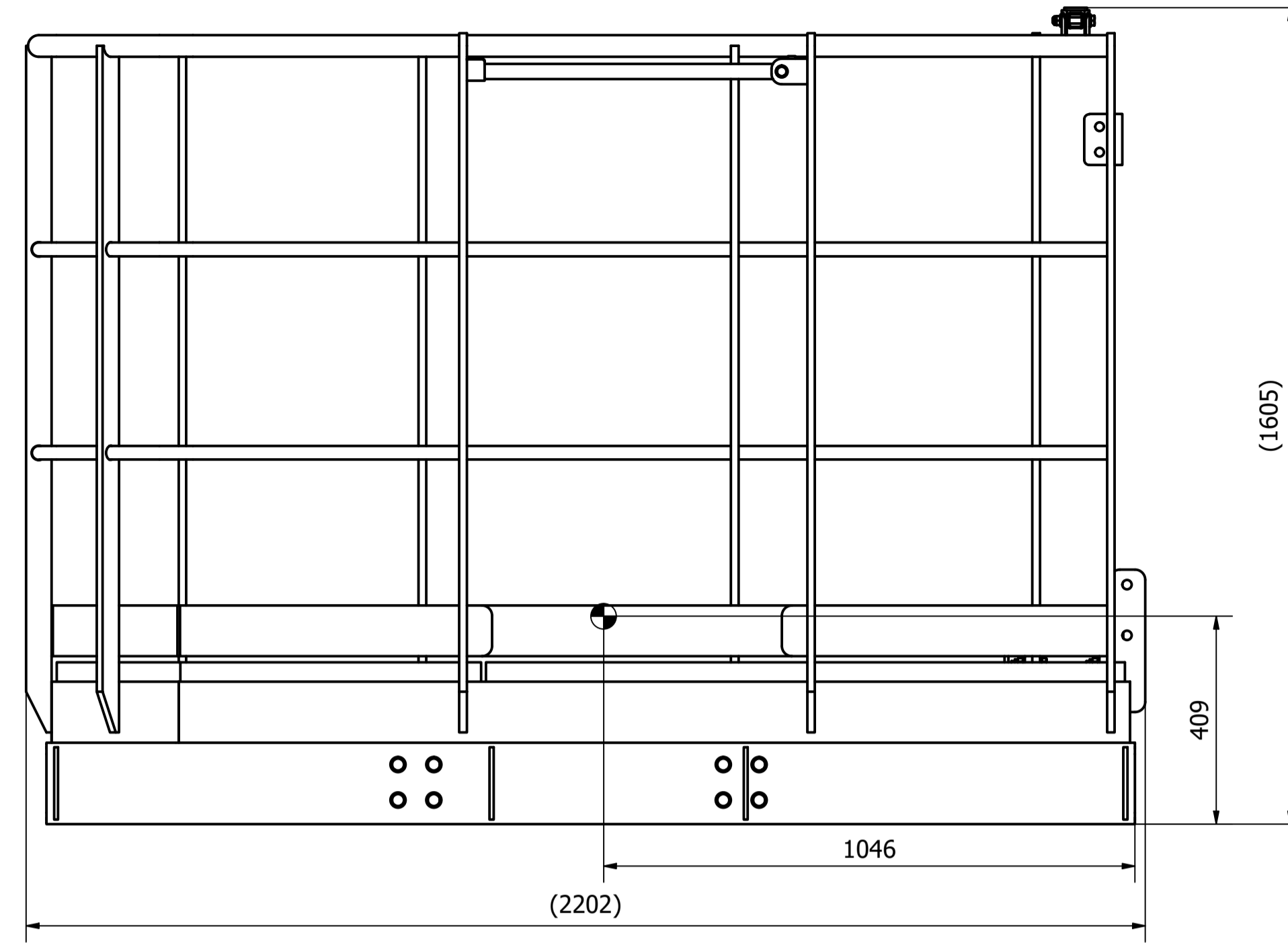
FRONT VIEW ( 1:10 )
