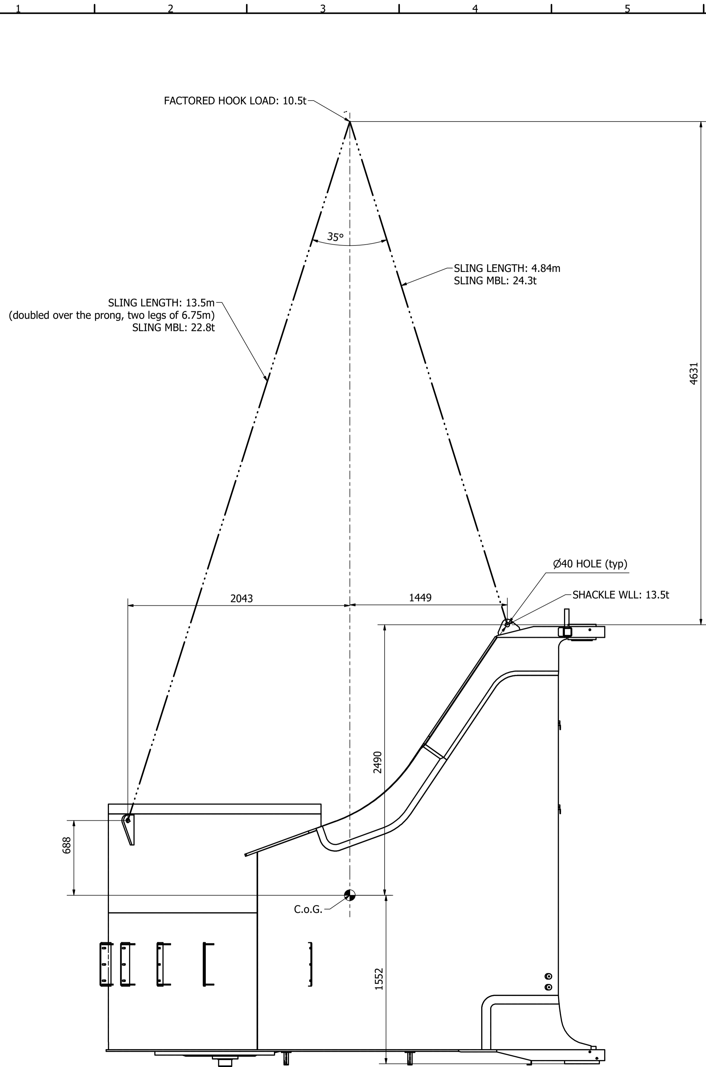
SIDE VIEW (1:20)
