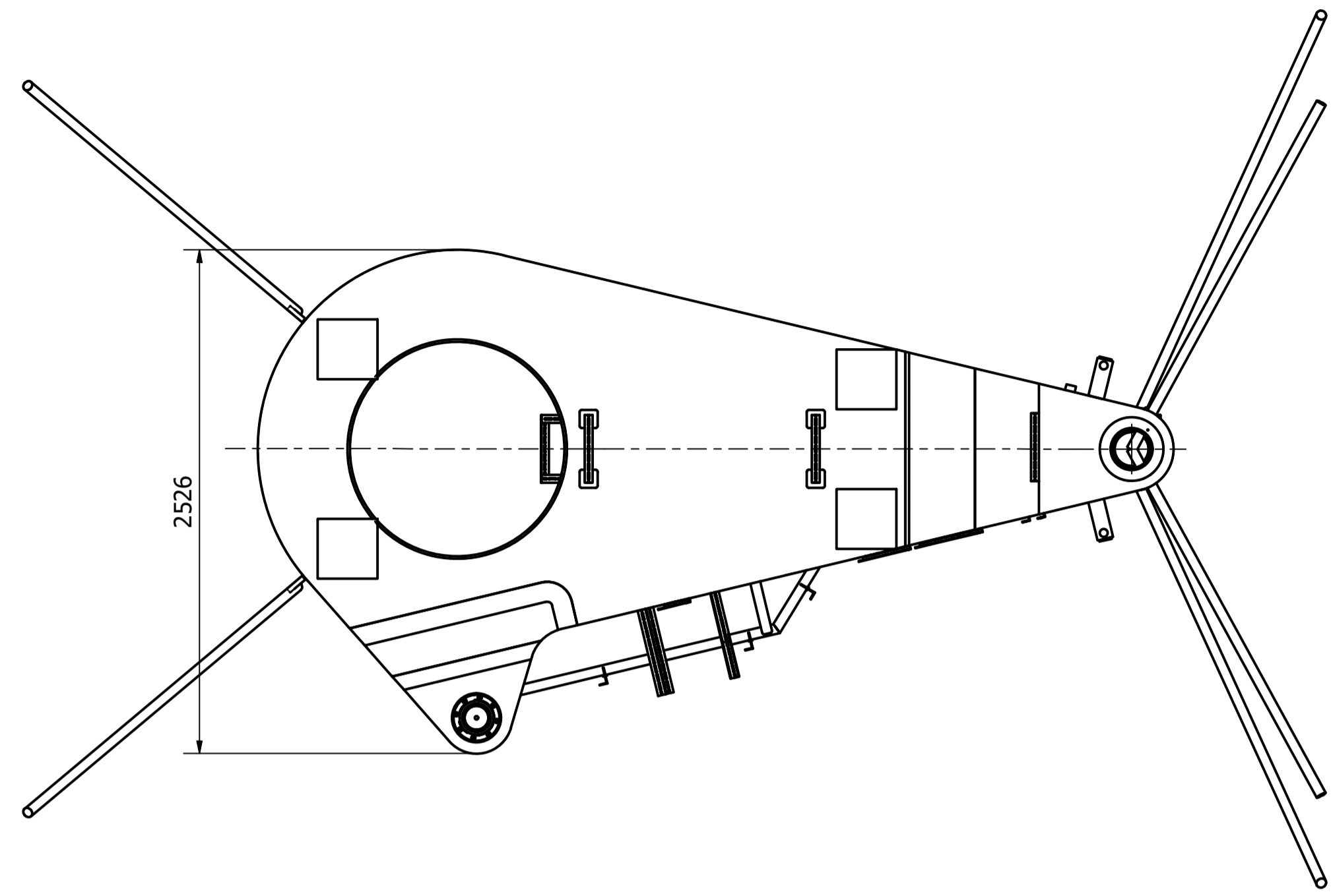
BOTTOM VIEW ( 1:25 )
