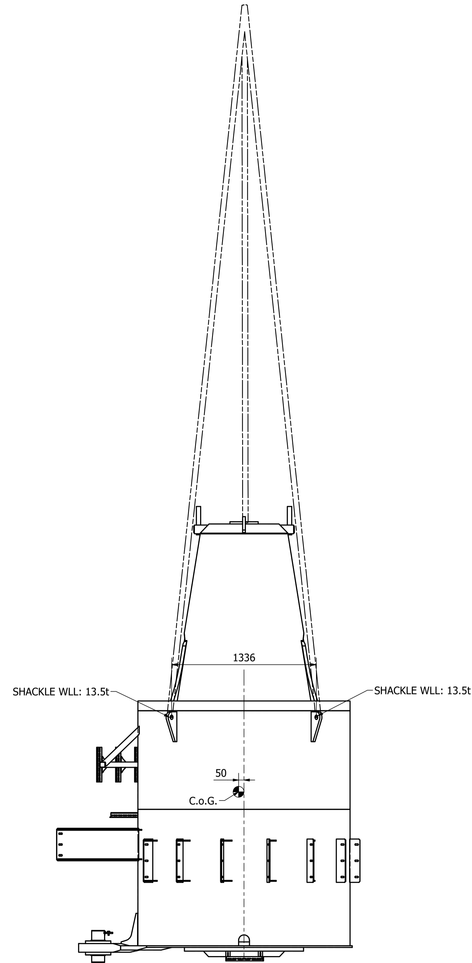
FRONT VIEW
