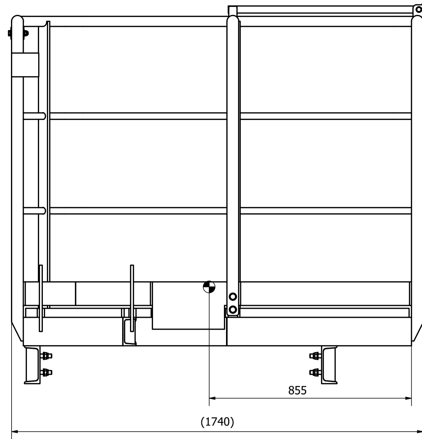
SIDE VIEW ( 1:10 )
