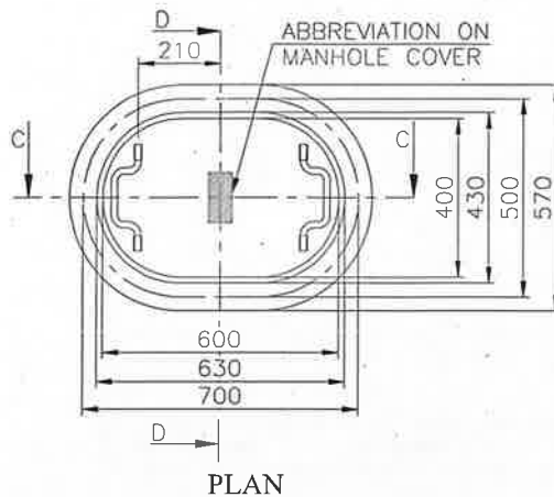
PLAN OVAL MANHOLE ABREAST STUD TYPE A
