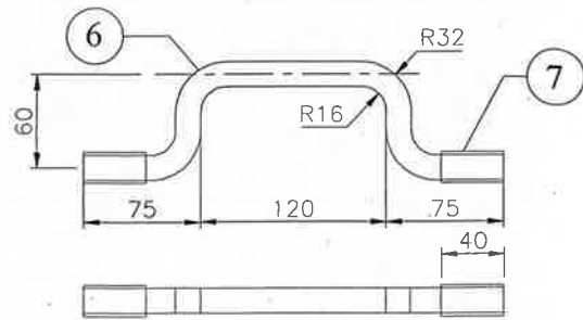
HANDLE DETAILS SCALE 1:5
