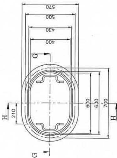
SECTION G-G SCALE 1:10
