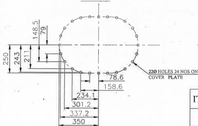
PLAN OVAL MANHOLE ABREAST STUD TYPE A
