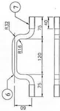
HANDLE DETAILS SCALE 1:5
