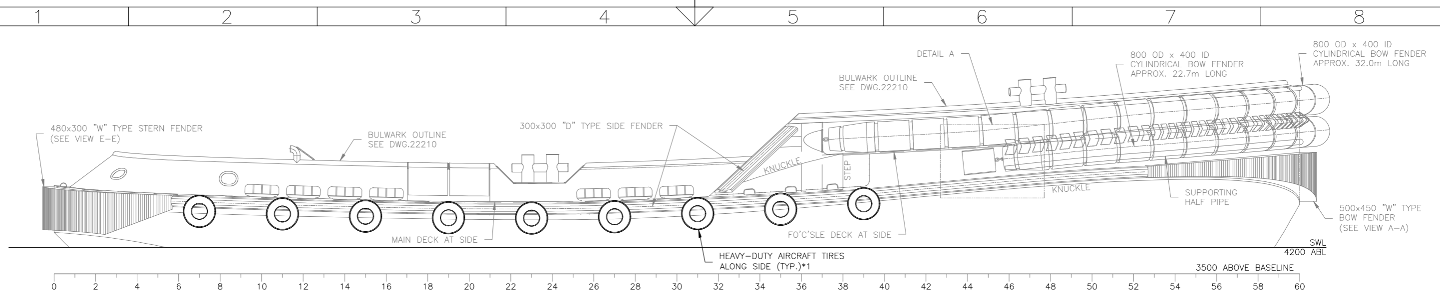
OUTBOARD PROFILE STARBOARD SIDE SHOWN, LOOKING TO PORT PORT SIDE SIMILAR
