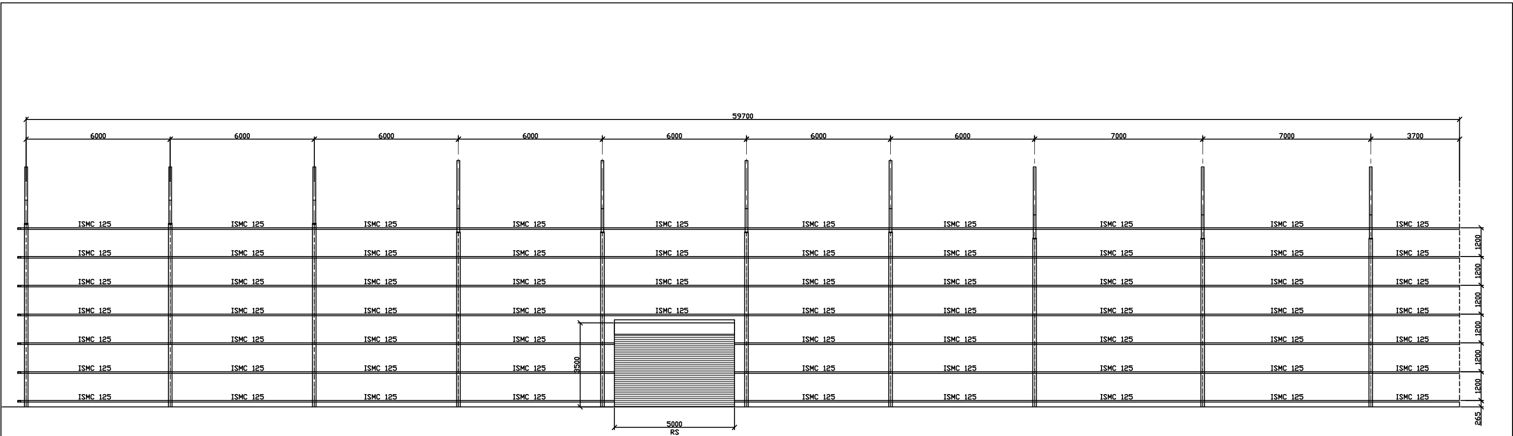
FRONT ELEVATION (VIEW @ A-A) (SHWN. VERTICAL PURLIN)
