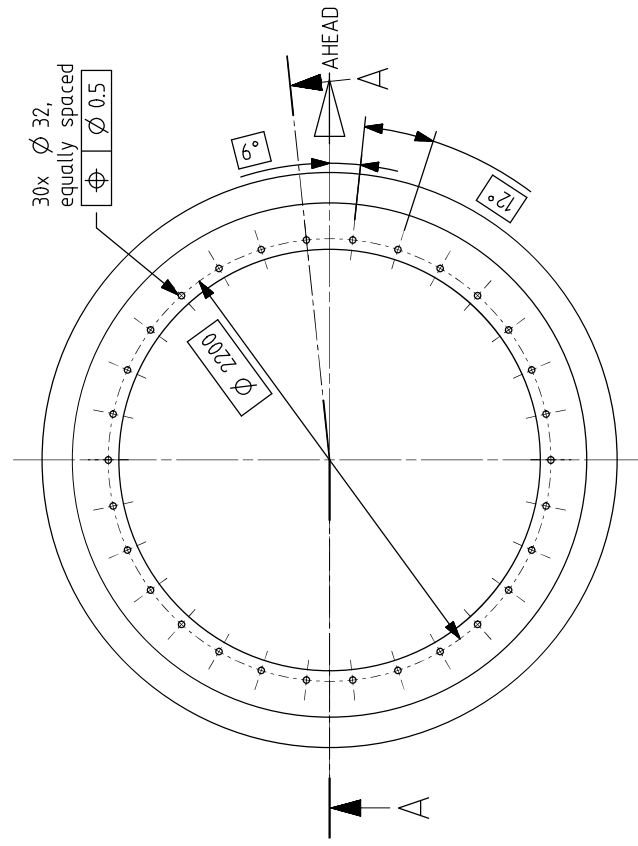
Hole pattern for vessel foundation
